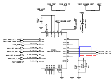
Audio amp
